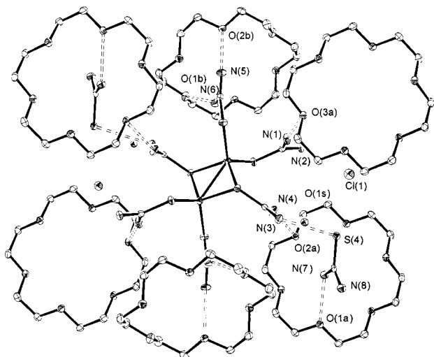
Fig. 2 The crystal environment of the [\text{Cu}_2\{\mu\text{-SC}(\text{NH}_2)_2\}_2\{\text{SC}(\text{NH}_2)_2\}_4]^{2+} cation in 4 . Selected intermolecular contacts ( \text{\AA} ): N(1) \cdots O(3a) 2.991(2), N(2) \cdots S(4) 3.350(2), N(3) \cdots S(4) 3.305(2), N(4) \cdots O(2a') 3.017(2), N(5) \cdots O(2b) 2.937(2), N(6) \cdots O(1b) 2.915(2), N(7) \cdots O(1a) 2.856(2), N(7) \cdots O(2a) 3.013(2), N(8) \cdots Cl(1) 3.278(2), N(8) \cdots Cl(1'') 3.409(2)
